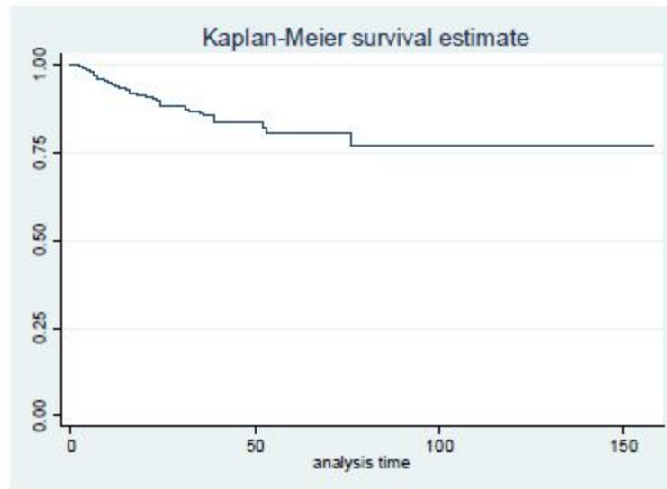
Figure 4: Survival Probabilities
